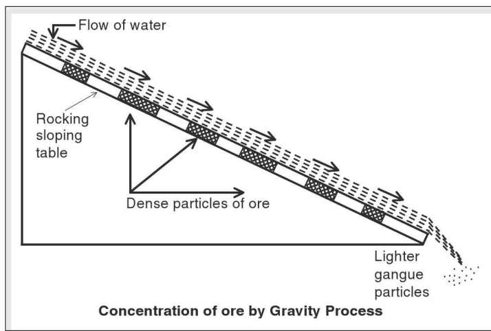
Figure 8.1 Concentration of ore by Gravity Process
