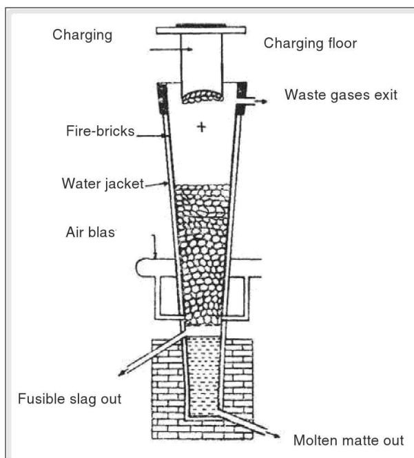
Figure 8.17 Blast furnace for copper
