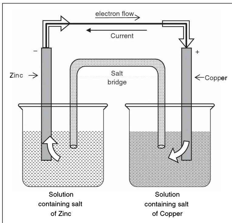
Figure 7.6 Schematic representation of Daniel cell
