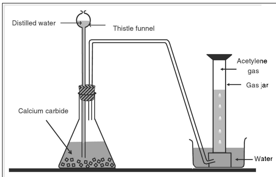
Figure 10.3 Preparation of acetylene gas
