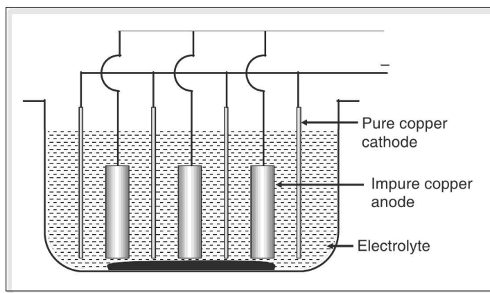
Figure 7.8 Anode mud or slime
