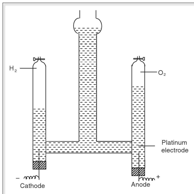
Figure 7.7 Hoffman's voltmeter
