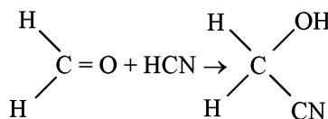
Methanal cyanohydrin
