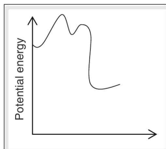
Figure 2.9 Reaction coordinate
