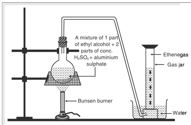
Figure 10.2 Laboratory preparation of Ethene
