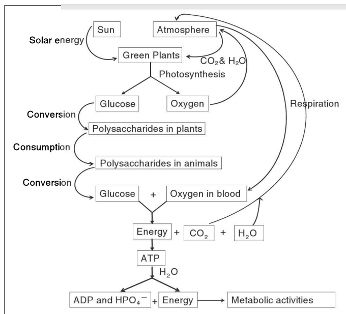
Figure 11.1 Energy cycle
