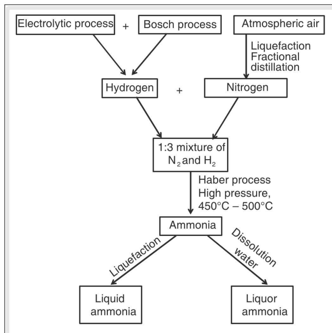
Figure 9.4 Flow chart for the manufacture of ammonia by Haber's process
