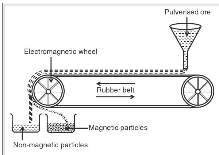
Figure 8.3 Electromagnetic separation
