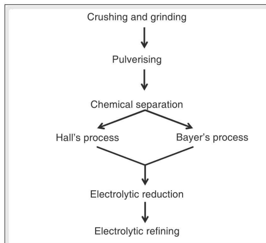
Figure 8.7 Process flow metallurgy of aluminium
