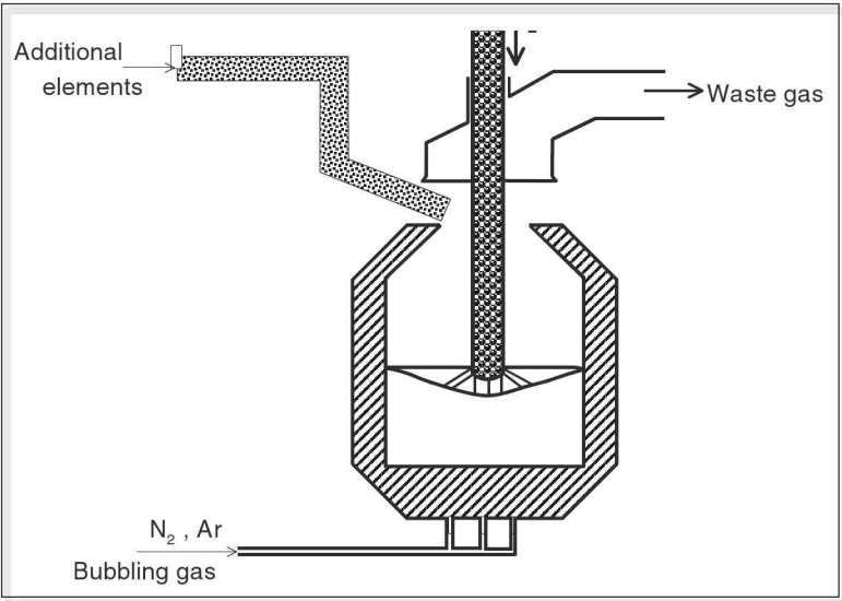
Figure 8.14 Schematic diagram of L – D converter
