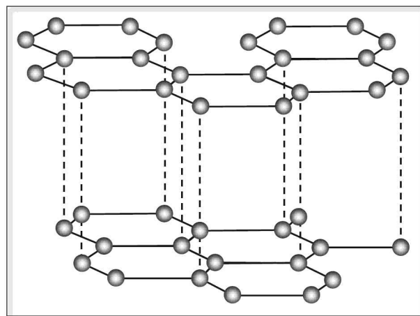
Figure 9.2 Structure of graphite
