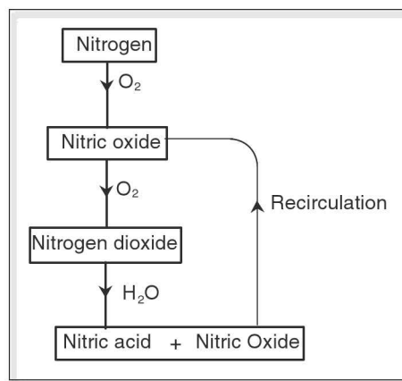
Figure 9.5 Flow chart for the manufacture of nitric acid by Oswald's process
