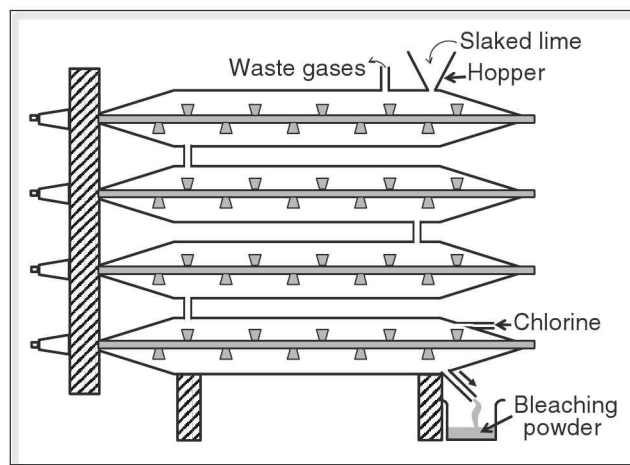
Figure 9.13 Hasenclever plant for the manufacture of bleaching powder
