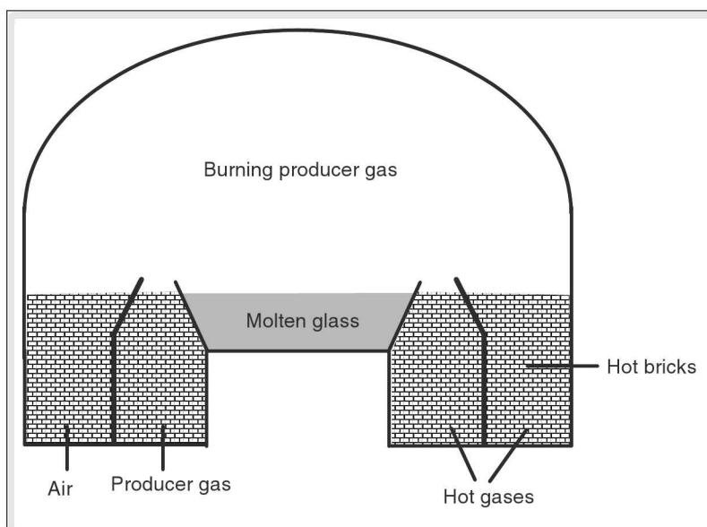
Figure 9.17 Manufacture of glass (tank furnace)
