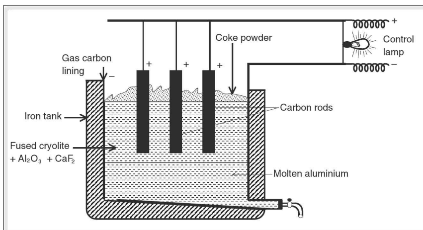
Figure 8.5 Electrolysis of fused alumina
