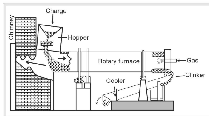
Figure 9.15 Rotary kiln
