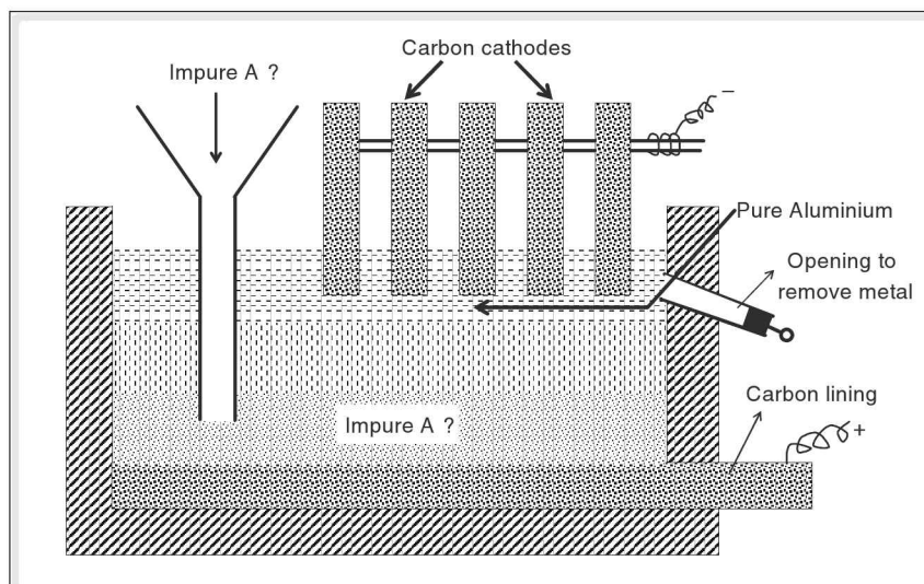
Figure 8.6 Refining of aluminium by Hoope's method
