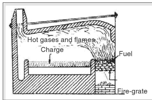
Figure 8.16 Reverberatory furnace
