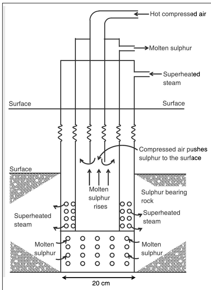
Figure 9.6 The Frasch process for extracting sulphur
