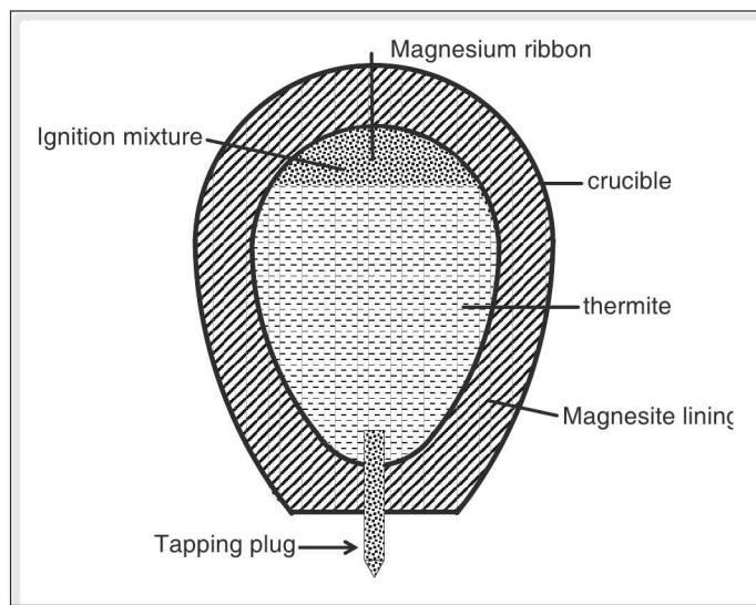
Figure 8.8 Aluminothermic process
