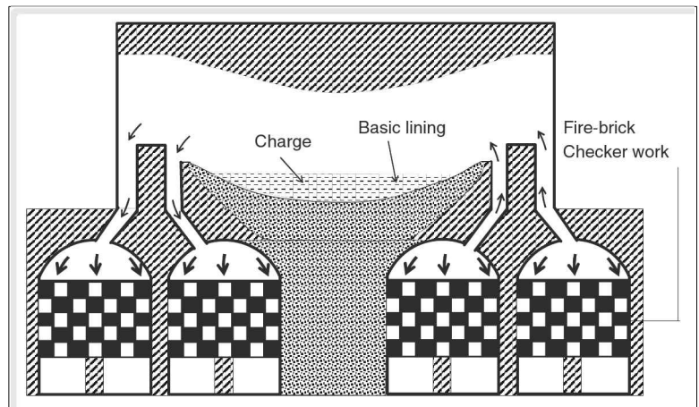
Figure 8.13 An open hearth furnace
