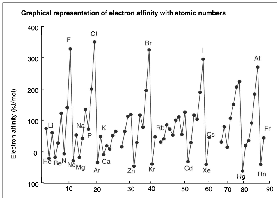
Figure 4.2 Atomic number
