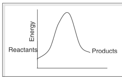
Figure 2.7 Course of reaction
