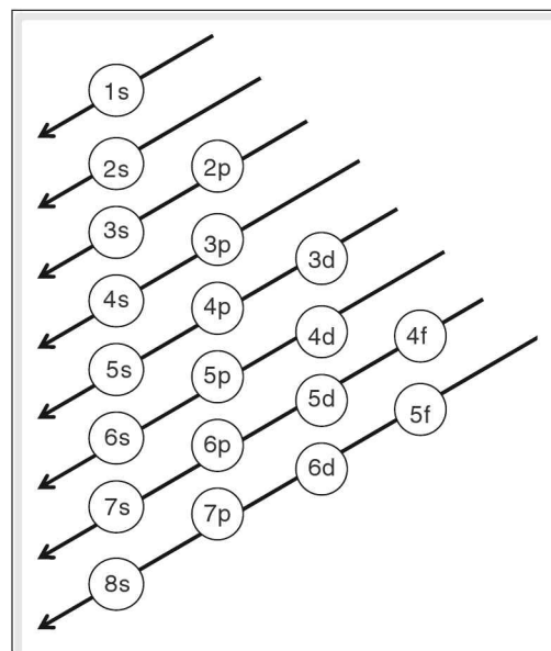
Figure 3.7 Moeller diagram
