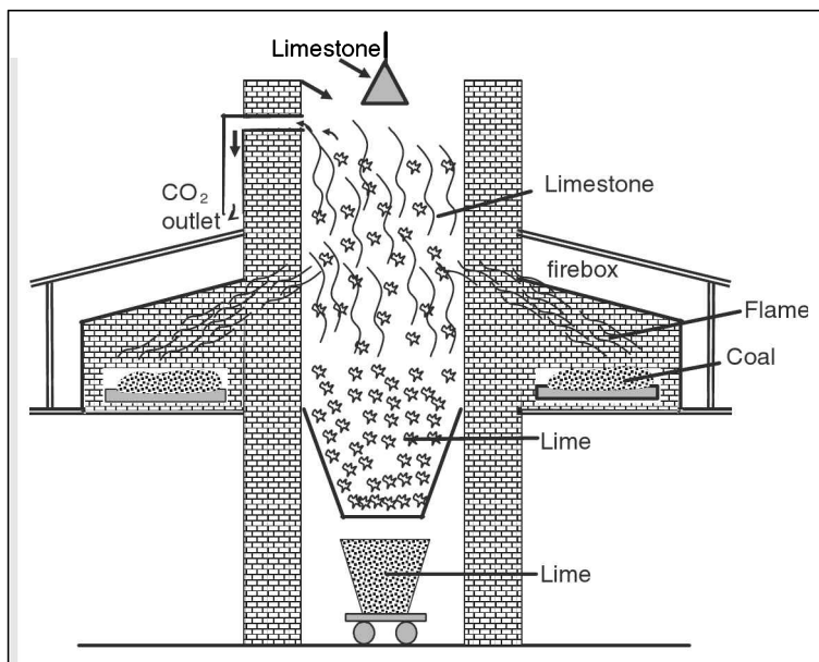
Figure 9.10 A vertical lime kiln
