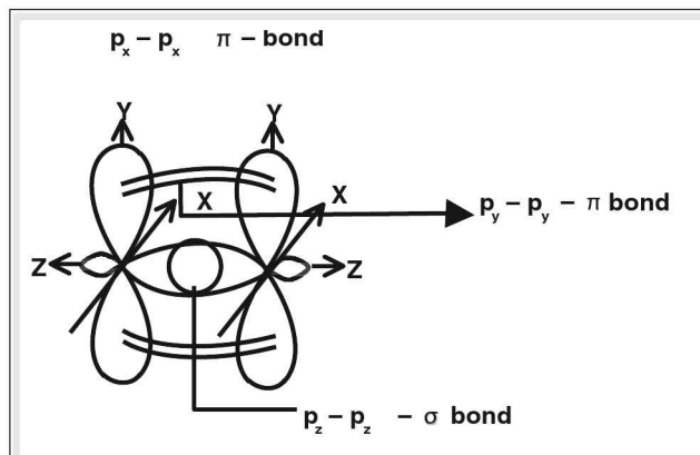
Figure 5.5 O 2 molecule (one \sigma bond and one \pi bond)
