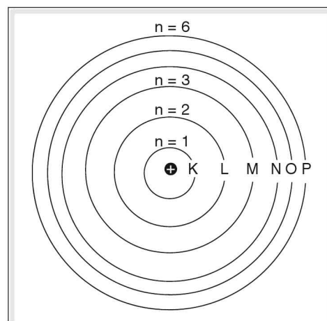
Figure 3.1 Stationary orbits of an atom
