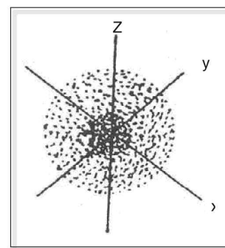
Figure 3.3 s-orbital
