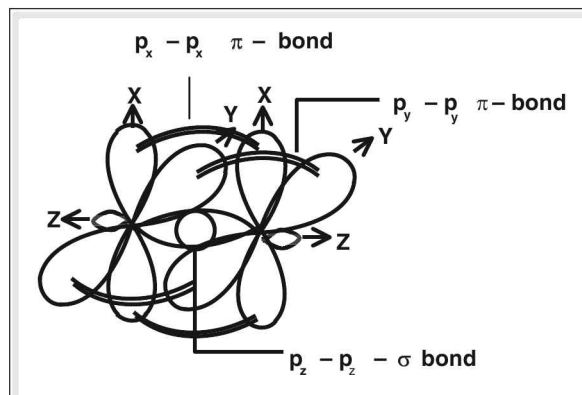
Figure 5.6 N 2 molecule (two \pi bonds and one \sigma bond)
