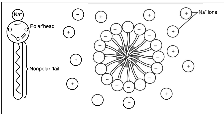
Figure 11.2 (a) A soap molecule (b) Cross section of a soap micelle in water
