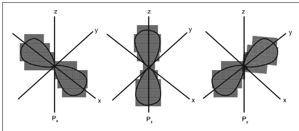
Figure 3.5 The boundary surface diagrams of the p orbitals
