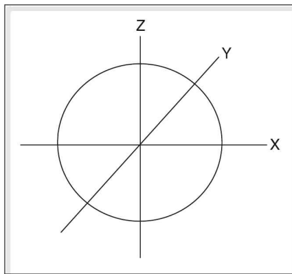
Figure 3.4 The boundary surface diagram of 1s orbital
