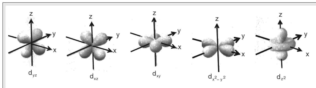
Figure 3.6 The boundary surface diagrams of five d-orbitals.
