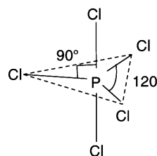
trigonal bipyramidal
