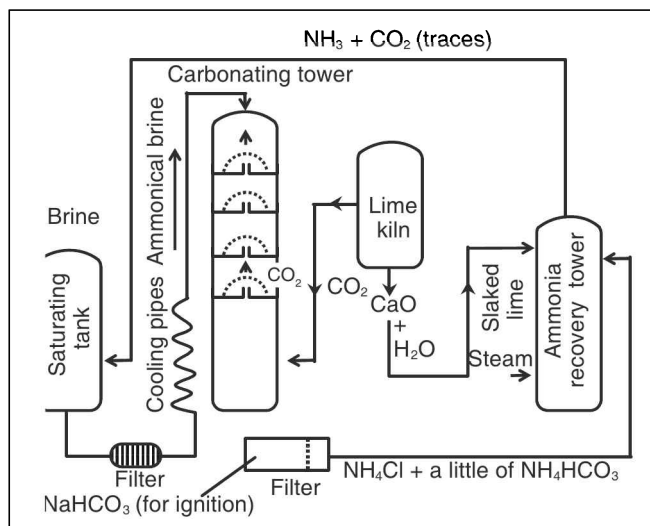
Figure 9.12 Flow diagram of Solvay process
