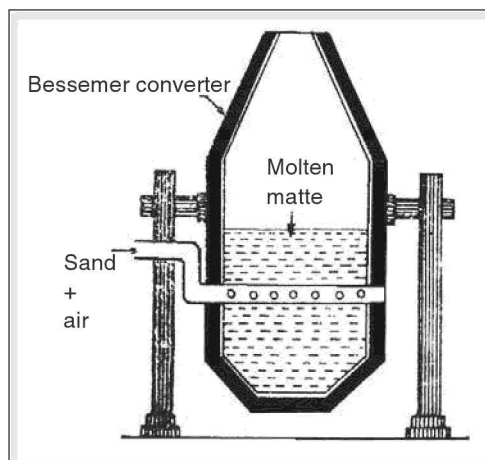
Figure 8.18 Bessemer converter for copper
