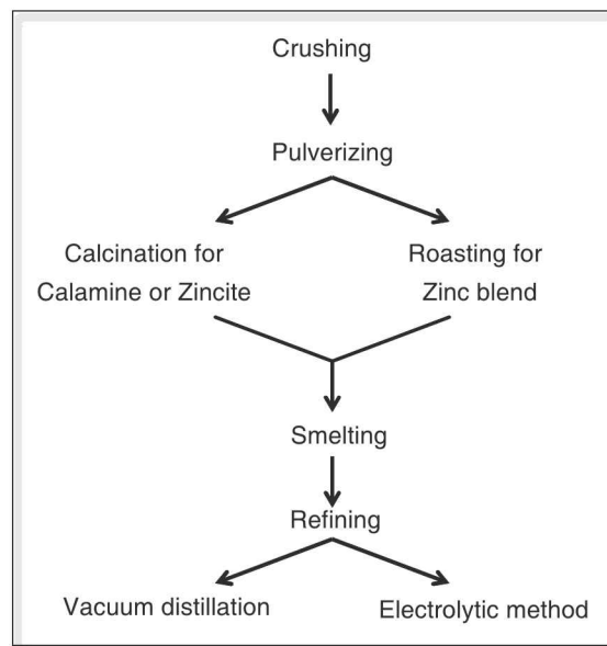
Figure 8.10 Process flow sheet for metallurgy of zinc
